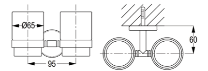
RAK21014 Double tumbler holder, glass wall fastening with screws and dowels
